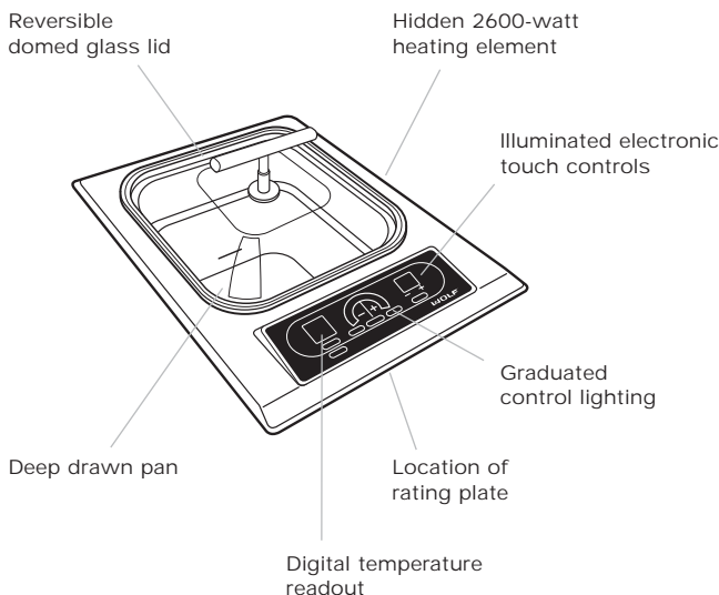
Model IS15/S
